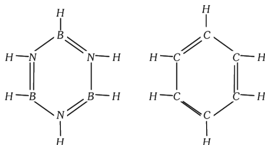
Borazine
